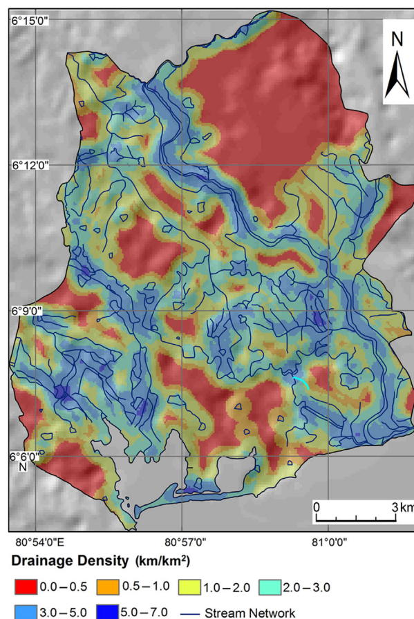
Figure 6. Drainage density map of Ambalantota.
