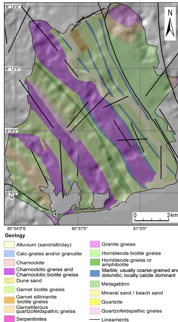
Figure 8. Lithological map of Ambalantota, Sri Lanka.
