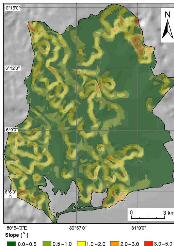
Figure 5. Slope map of Ambalantota, Sri Lanka.
