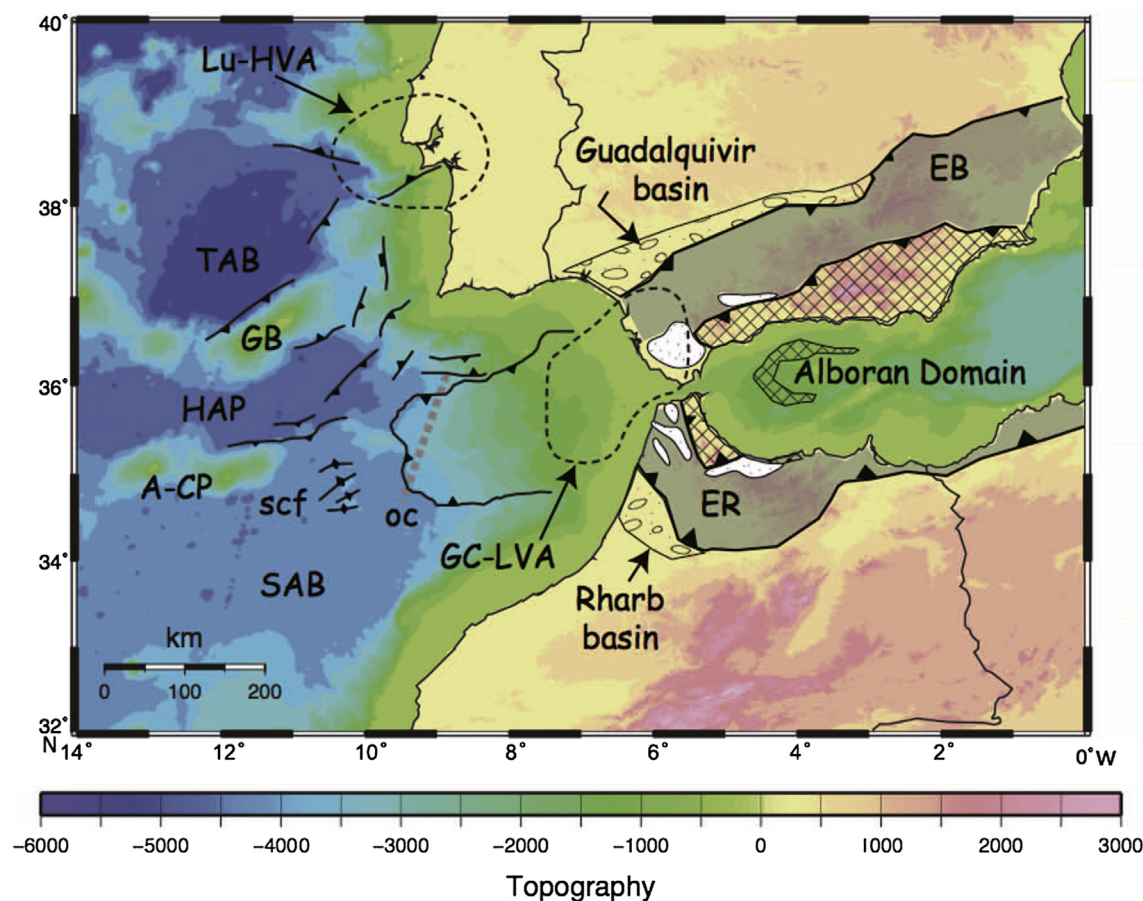
Figure 2. Simplified geological map of the study area (after Gutscher et al., 2012; Duarte et al., 2013; Platt et al., 2013). The Alboran domain is indicated by cross hatched pattern. The External Betics (EB in gray pattern) includes the Subbetic and Prebetic, and the External Rif (ER in gray pattern) includes the Intrarif and Mesarif. The white field with dotted pattern represents the Flysch belt. The gray dashed line indicates the extent of oceanic crust (oc) inferred from refraction seismic (Sallarès et al., 2011). The approximate location of the Lu-HVA (at about 400 km depth) and of the GC-LVA (100–200 km depth) is also indicated. A-CP = Ampere-Coral Patch seamounts. TAB, GB, HAP, and SAP are as in Fig. 1.
