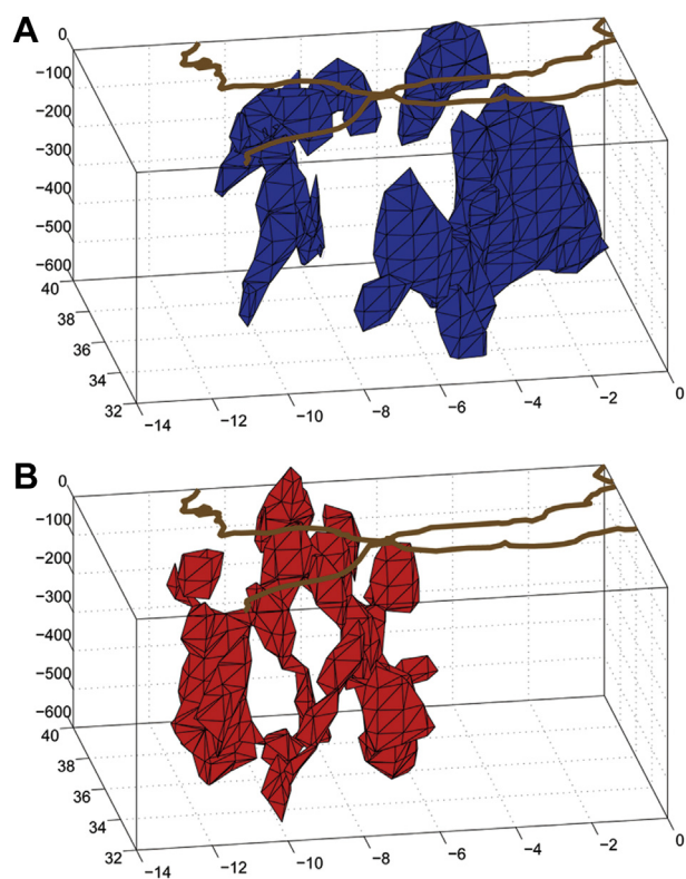
Figure 6. Three-dimensional perspective view (azimuth 200°, elevation 30°) of the high velocity (A) and low velocity (B) isosurfaces extracted from the 3D model. Isosurfaces are drawn at \pm 0.07 km/s velocity perturbations relative to the reference values. Note the complex morphology of the Alboran subduction zone moving along the pronounced arcuate shape of the Betics and Rif mountain belts. West of Gibraltar Strait, the 3-D visualization shows well-developed slow structures which interrupt the lateral continuity with the Atlantic high velocity anomaly.
